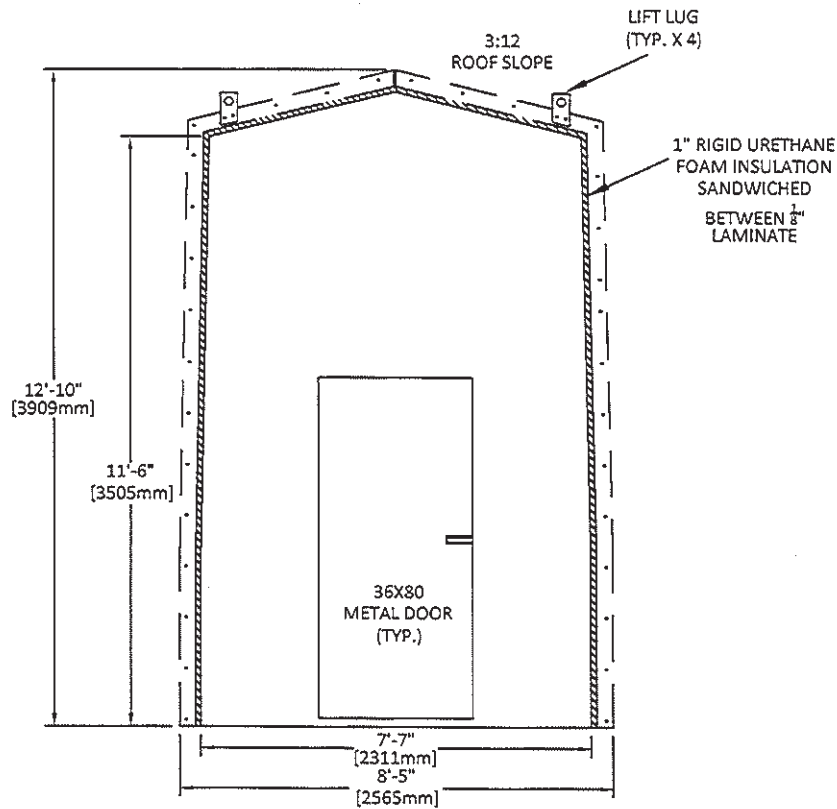
FRONT ELEV.
