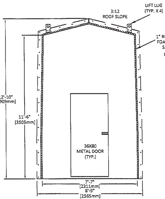
FRONT ELEV.
