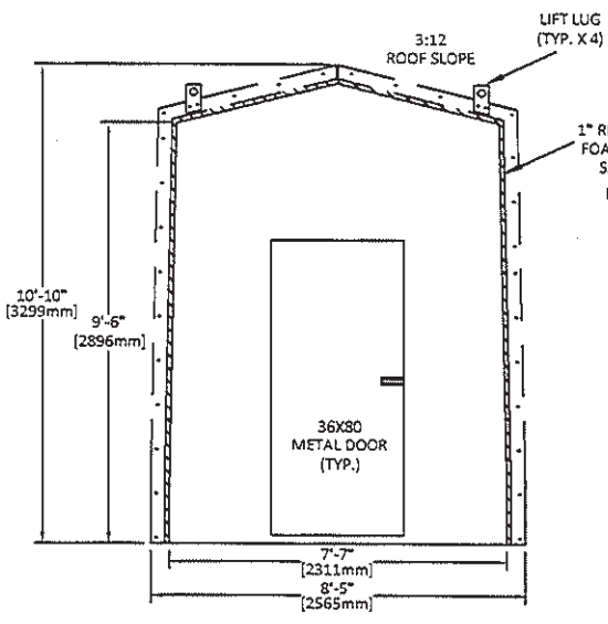
FRONT ELEV.
