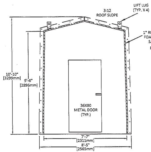
FRONT ELEV.
