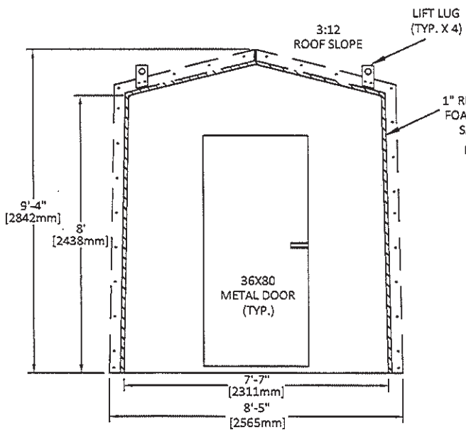
FRONT ELEV.
