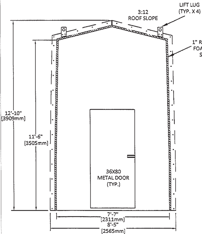
FRONT ELEV.
