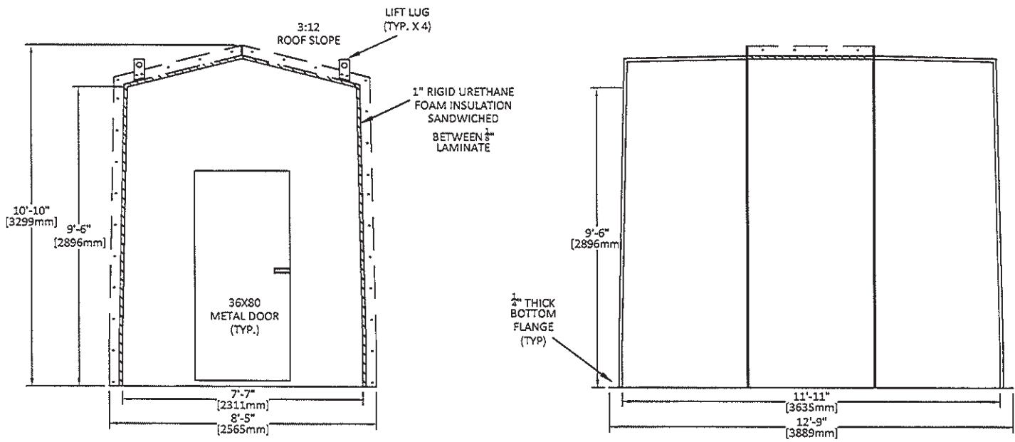
FRONT ELEV.
