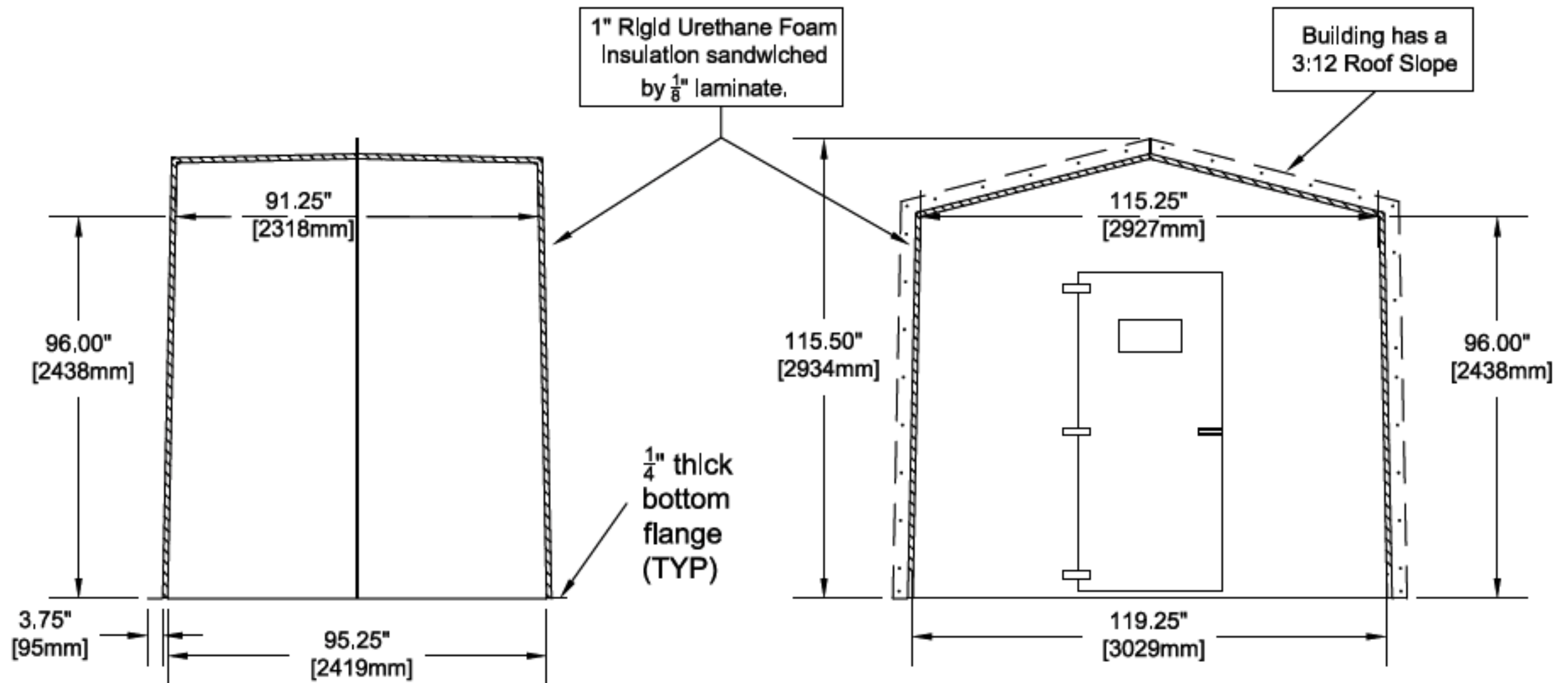
SIDE VIEW
