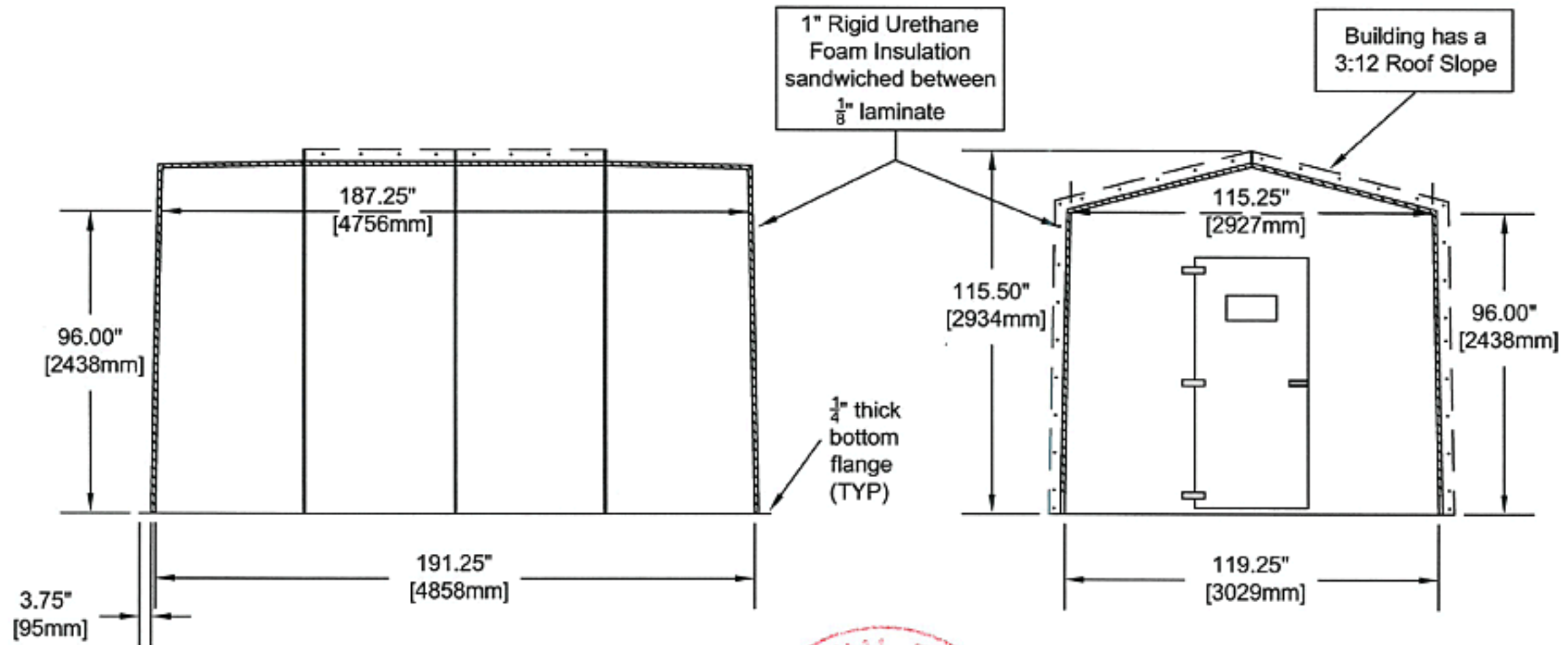
FRONT VIEW
