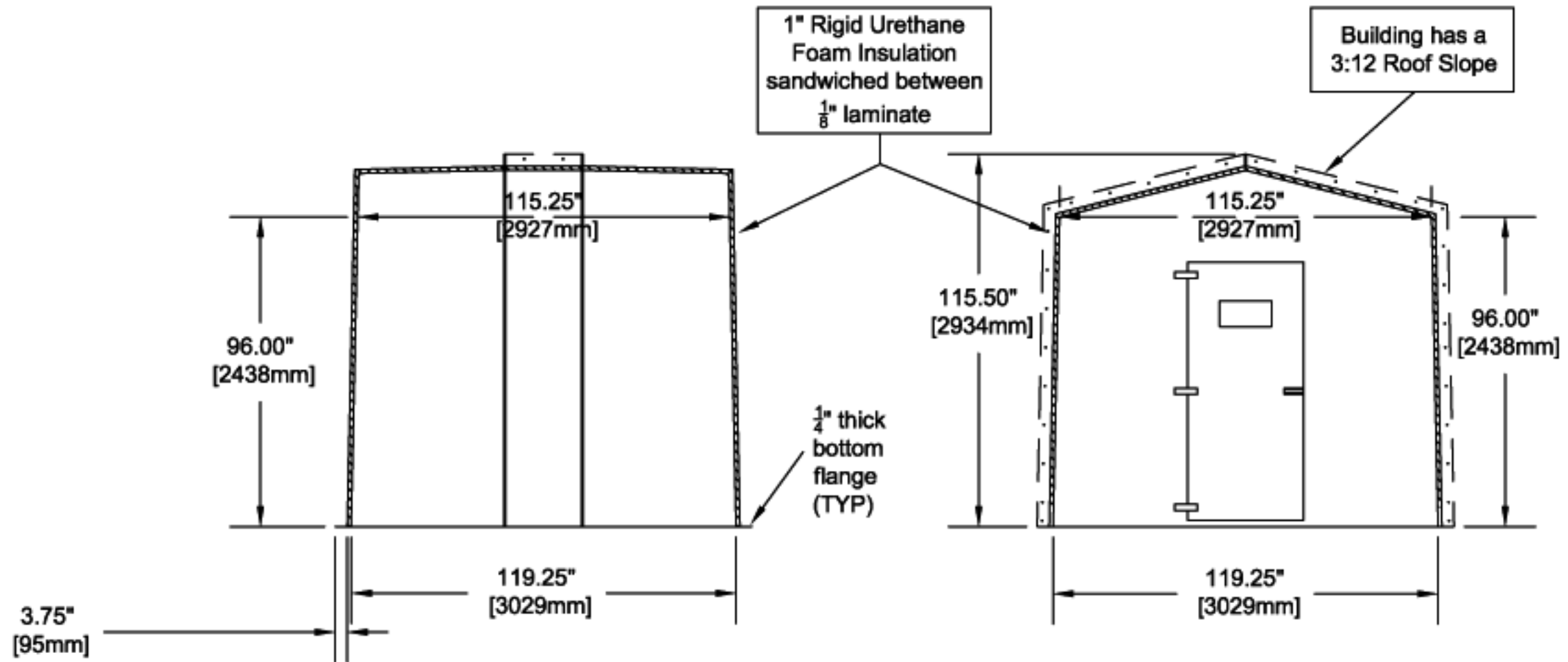
SIDE VIEW
